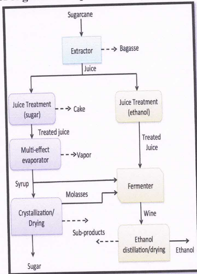
H) Figure 7.4: Schematic of process of sugarcane to produce ethanol and sugar.
